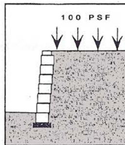
Level Backfill 100 psf Surcharge
