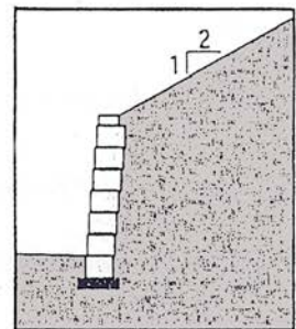
Sloping Backfill 2H:1V Maximum
